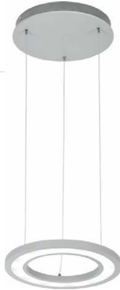
6387 LOOP LED GRAY M ↓ 68 cm Ø 29 cm 18W, ~230V, 50Hz 4000K, 1800lm
